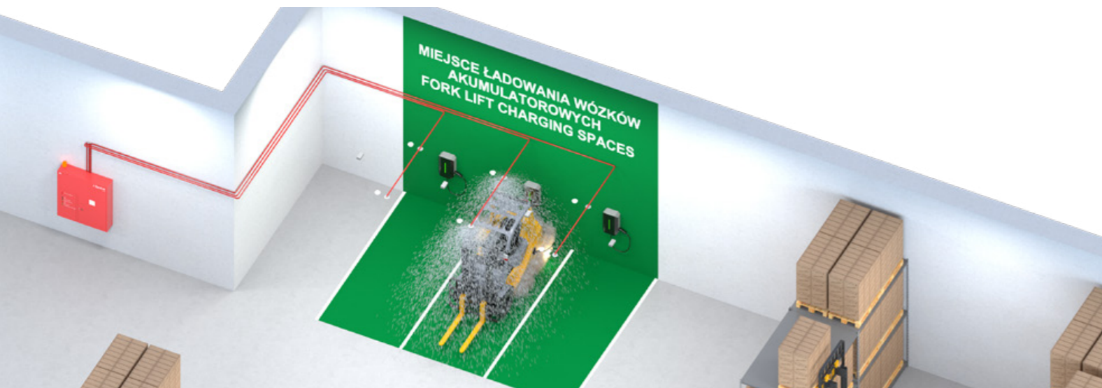
i-Sprink type kit used to protect parking and charging spaces for battery-operated forklift trucks in the warehouse building
